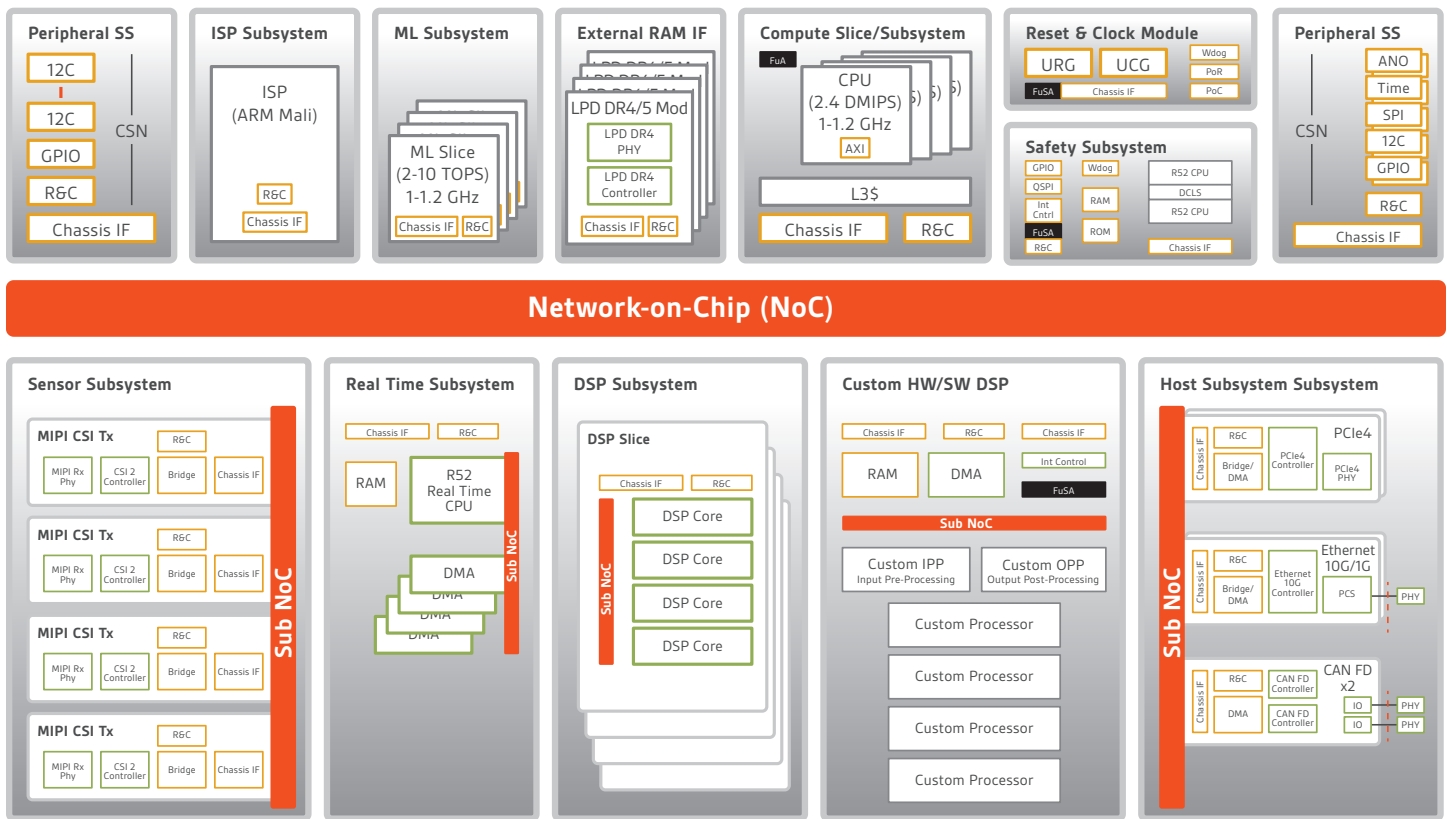
Figure 1. Aion Silicon SFA 350A Chassis
