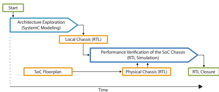
Figure 2. Shifting NoC Performance Verification Left
